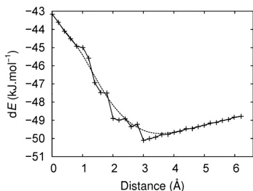
Fig. 4. The electrostatic free energy of interaction is plotted as a function of distance between the van der Waals surfaces of protein and membrane atoms and was determined by solving the Poisson-Boltzmann equation for the HgACBP/membrane system. Zero distance is defined as the configuration in which protein and membrane van der Waal atom surfaces are in contact. In each of the dE calculations, the protein orientation with respect to the membrane remained fixed and only the protein–membrane relative distance ( r ) was varied. The dashed line shows an approximation with a minimum between 3 and 4 Å.
